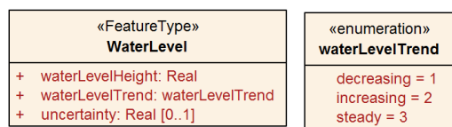
Figure 4-1 – Water level feature
