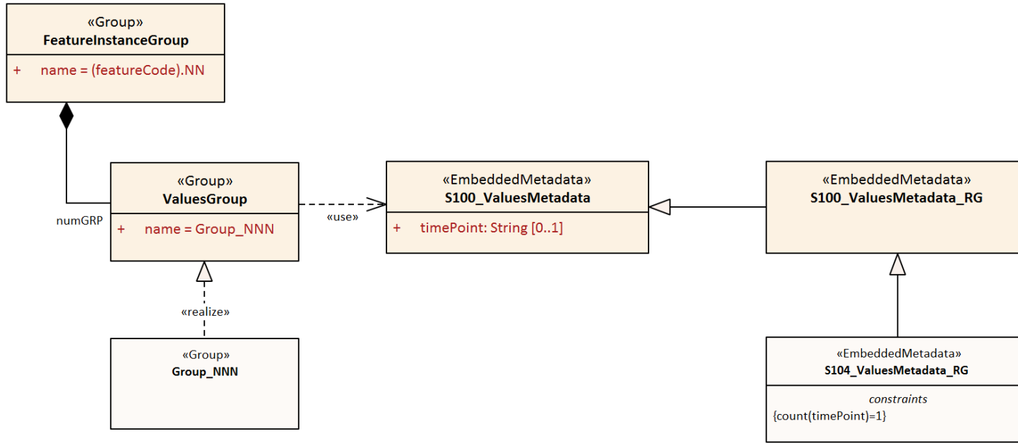
Figure 12-9 – Feature Instance metadata – Carrier metadata for the Values group in each Feature Instance group
