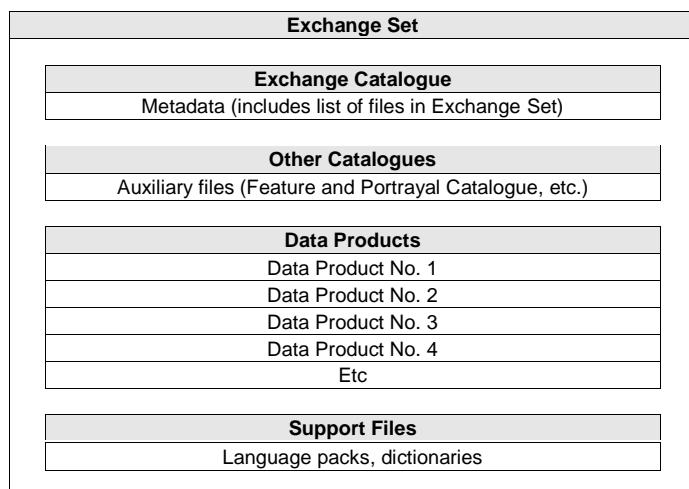
Figure 11-1 – Schematic diagram of the Exchange Set.
