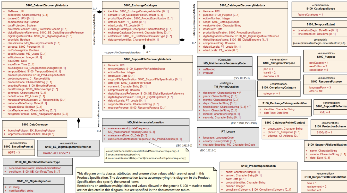
Figure B-5 – Exchange Set class details
