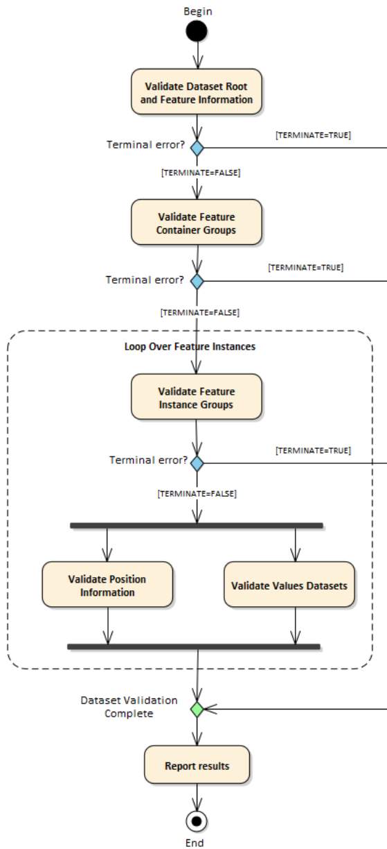
Figure E-1 – Phases of dataset validation processing
