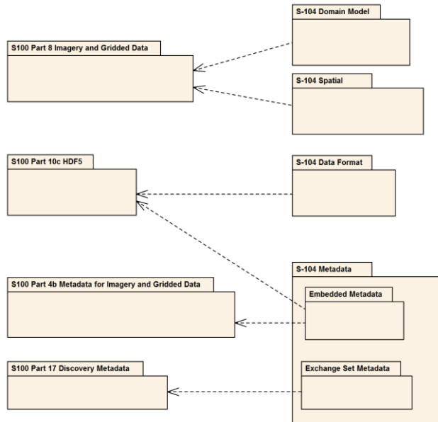
Figure B-2 – Derivations from S-100
