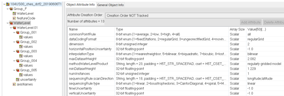
Figure D-3 – General structure of dataset (expanded on left) and attributes of feature type group (on right)
