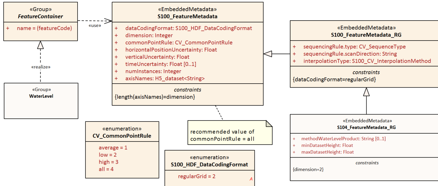
Figure 12-7 – Feature Type metadata – Carrier metadata for the Feature Container group
