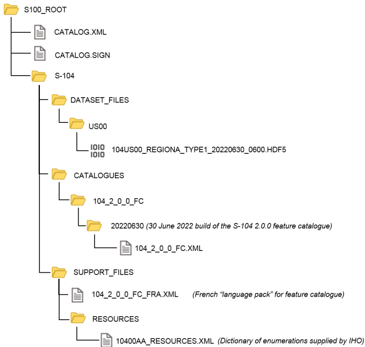
Figure 11-2 – Typical Exchange Set structure
