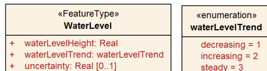
Figure B-4 – Domain Objects
