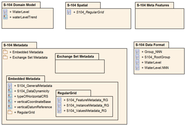
Figure B-1 – S-104 Model components
