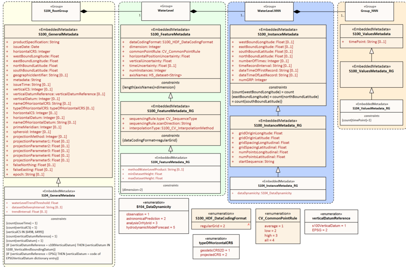
Figure B-6 – All carrier metadata for coverage type Regular Grid (data coding format 2)
