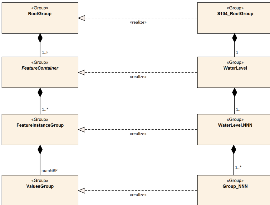
Figure 10-1 - Outline of the data file structure for S-104 data files, showing the realisation of S-104 structure from the generic structure described in S-100 (see S-100 Part 10c, Figure 10c-7). Note that there are four levels from top to bottom
