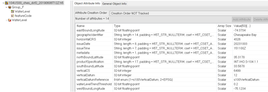
Figure D-1 – Typical root group structure and attributes
