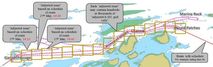
Figure F-2 – Adjustment zones based on planned route (courtesy: Furuno Electric Company, Ltd)
