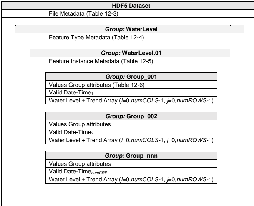
Figure 10.2 - Schematic of the S-104 HDF5 data product structure. The four parameters numPOS, numCOLS, numROWS, and numGRP are explained in Table 10-5.
